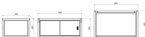
Anti-draft chamber for microbalances
