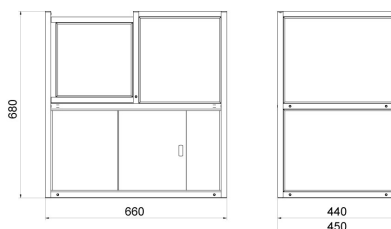
Anti-draft chamber for APP-KO-SK mass comparators
