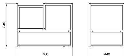
Anti-draft chamber for APP-00-SK mass comparators
