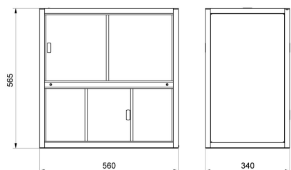
Anti-draft chamber for WAY-KO-SK mass comparators
